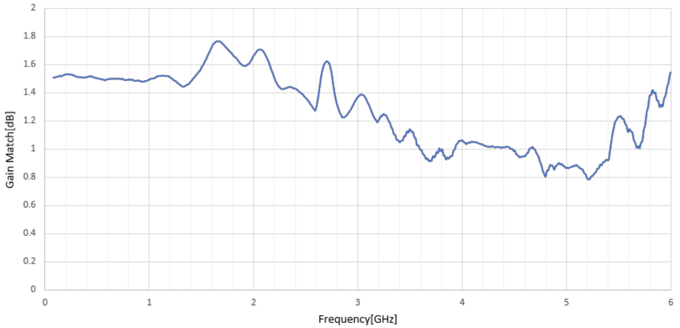
Overall Gain Deviation (Max - Min) in 100MHz to 6GHz Spec: \pm 2.5\text{dB}
