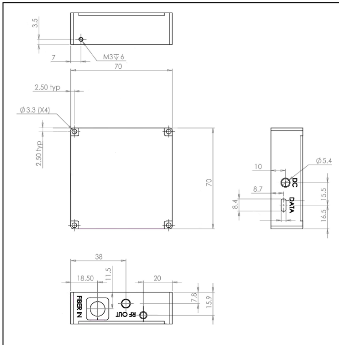
Rx unit
